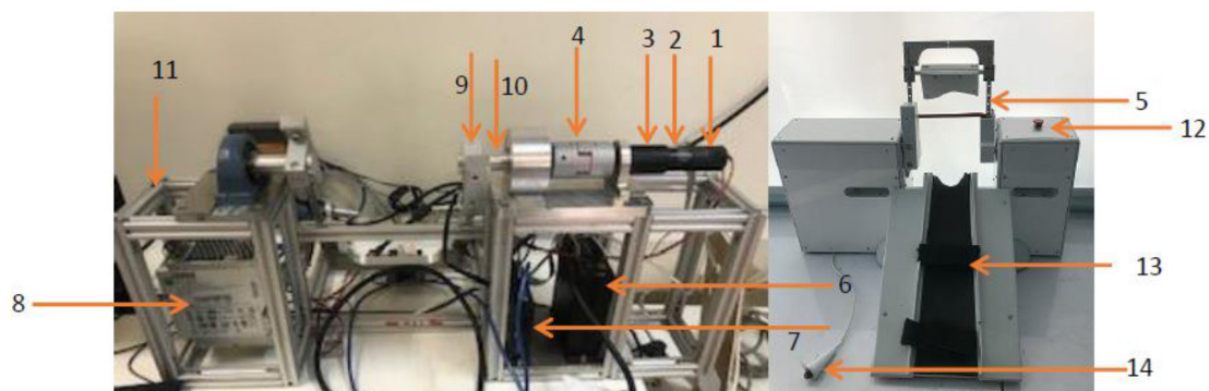
Figure 2: The robot platform 1: Encoder, 2: Direct-Current motor, 3: Reduction gearbox, 4: coupling mechanism, 5: Linear Guide, 6: Amplifier, 7: Position controller, 8: power supply, 9: load-cell, 10: Ball bearing, 11: mechanical structures, 12: Emergency stop, 13: Handset, 14: Emergency stop button
