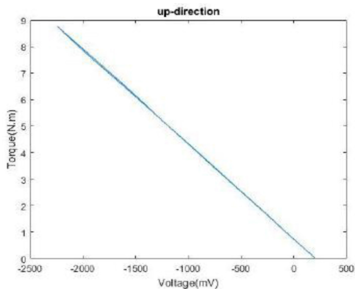
Figure 5: Diagrams of the calibrating loadcell in the opposite direction of force imposing
