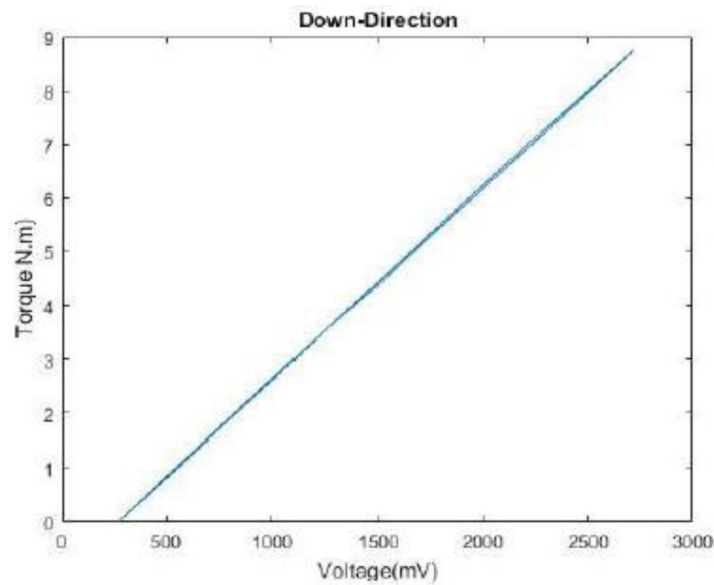
Figure 4: Diagrams of the calibrating loadcell in its real direction of force imposing
