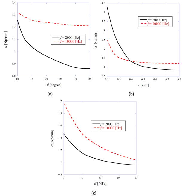
Figure 3: Structural dependency of attenuation constant of Reissner's membrane (RM) mode on (a) angle \theta between RM and basilar membrane (BM), (b) radius r of the cochlea, and (c) Young's modulus E of RM.
