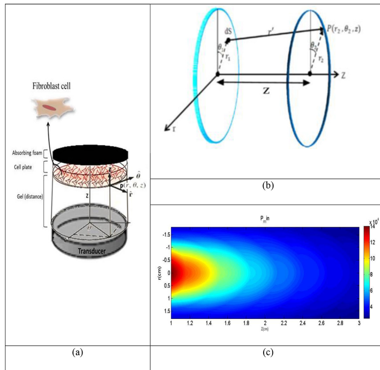
Figure 1: The acoustic pressure model of low-frequency ultrasound: a) the setup of the transducer and cell culture plate, absorbing foam prevents the creation of standing waves, b) geometry in the modeling in cylindrical coordinates, and c) the axial contour [r \text{ (cm)}] of acoustic pressure [P_m] .
