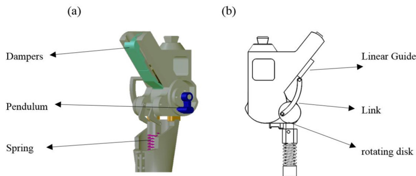
Figure 2: (a) The mechanical structure of the novel knee prosthesis, (b) the rotational force transform into the linear force via a link part
