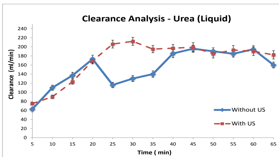
Figure 3: Effect of ultrasound on Urea clearance from blood equivalent solution
