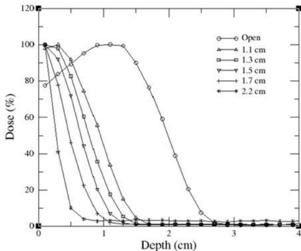
Figure 5: PDD curves for 5 MeV electron beam for 20 \times 20 \text{ cm}^2 , open field and different thicknesses of spoiler.
