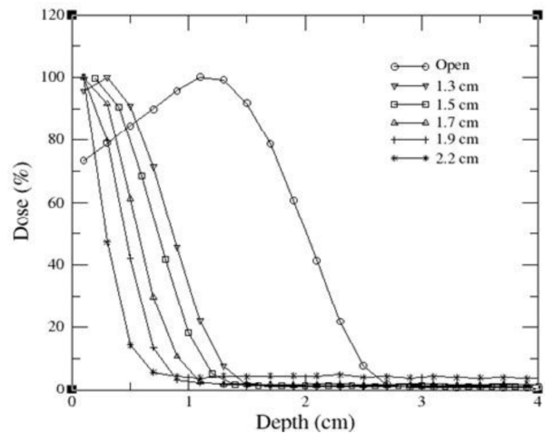
Figure 4: PDD curves for 5 MeV electron beam for 10 \times 10 \text{ cm}^2 , open field and different thicknesses of spoiler.
