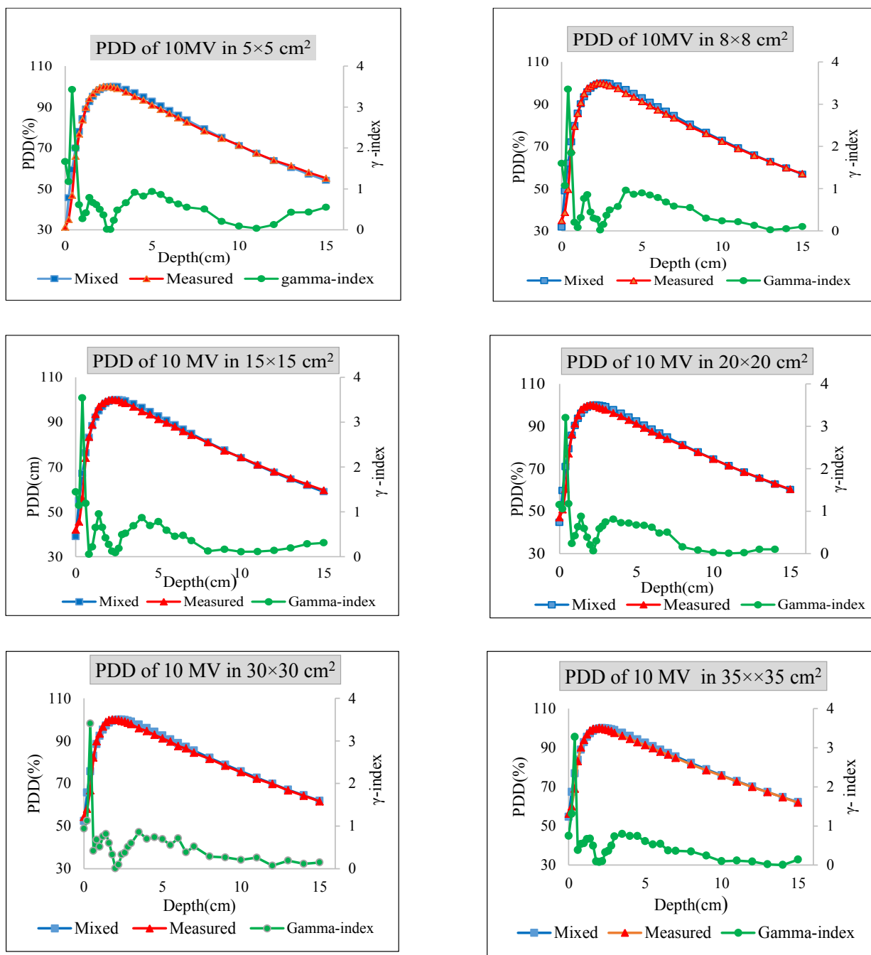
Figure 3: The comparison of calculated (weighing factor \alpha=0.43 ) and measured PDDs of 10 MV for 5×5, 8×8, 15×15, 20×20, 30×30, and 35×35 cm 2 .
