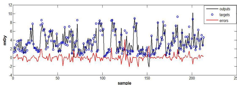
Figure 6: Comparing the neural network estimation (black), the collected data (blue), and the error value (red).
