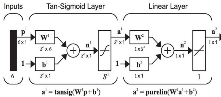
Figure 1: The bilayer neural network with six inputs and tangent sigmoid transfer function and one output with purelin transfer function.
