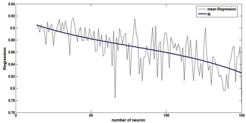
Figure 2: The output and target regression in relation to the number of neurons of the hidden layer.
