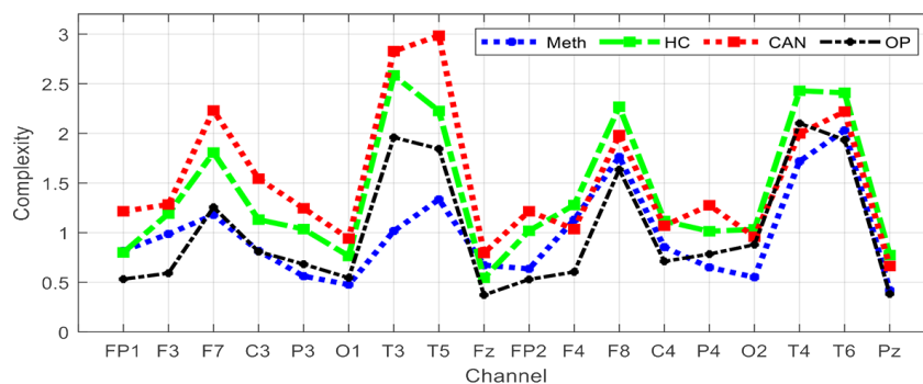
Figure 1: Mean complexity index values across Electroencephalogram (EEG) channels
