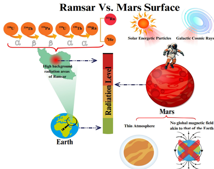
Figure 1: Comparison of the annual radiation dose in Ramsar, Iran, with that of the Martian surface.
