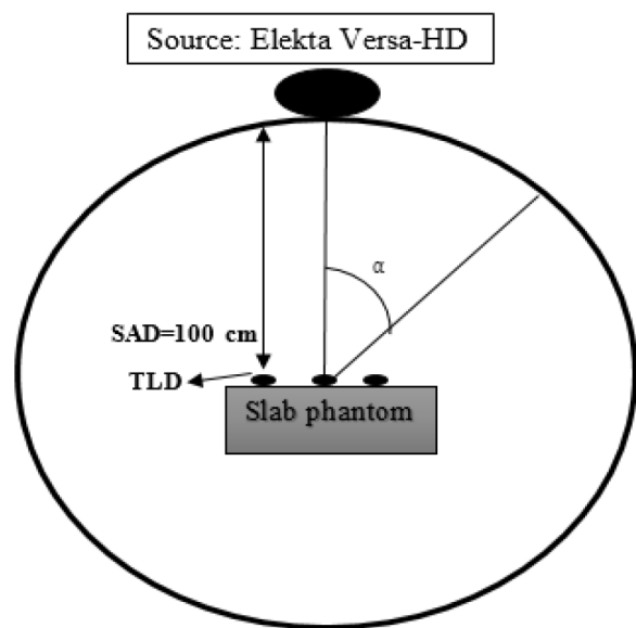
Figure 1: Schematic of the Thermoluminescent Dosimeter (TLD) 100 & GR200 uncertainty measurement set up: Elekta Vrsa-HD Linac, 6, 10, and 18 MV energies at different gantry angles (0, 20, 40, and 60), Source-to-Axis Distance (SAD)=100 cm.
