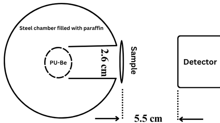
Figure 2: Experimental schematic of neutron irradiation of samples
