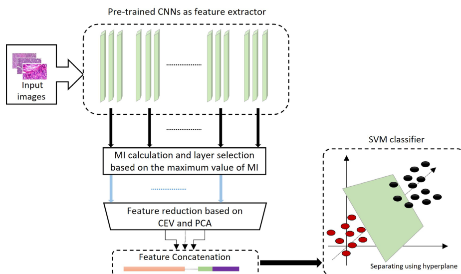
Figure 2: The diagram of the proposed method (Convolutional Neural Networks (CNNs), Mutual Information (MI), Cumulative Explained Variance (CEV), Principal Component Analysis (PCA), Support Vector Machine (SVM)).
