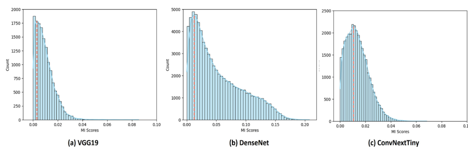
Figure 4: Histogram of Mutual Information (MI) scores for 100× magnification: (a) B4C4 layer in VGG19, (b) D3B32_2 layer in DenseNet, and (c) S3B2C layer in ConvNextTiny, where the red dashed line indicates the mode.
