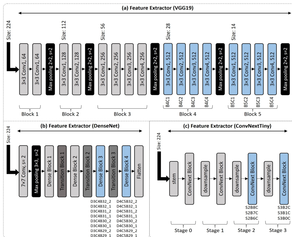
Figure 3: Investigated layers in the (a) VGG19, (b) DenseNet, and (c) ConvNextTiny networks. The blocks used for feature extraction are highlighted in blue, and the names of the layers in each block are indicated.
